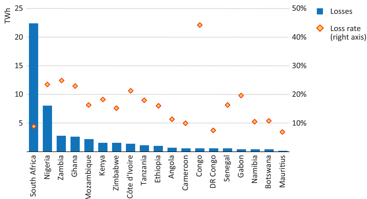
Figure 1.16 ▶ Transmission and distribution losses and loss rates, 2012
