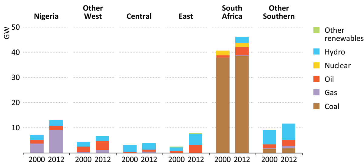
Figure 1.17 ▸ Installed grid-based capacity by type and sub-region
