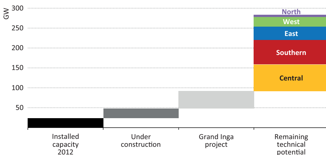
Figure 1.24 ▷ Existing hydropower capacity and potential in Africa
